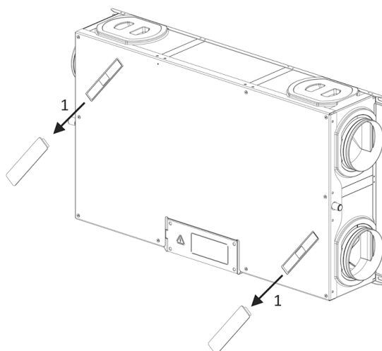
Illustration 6. Removing filter covers
