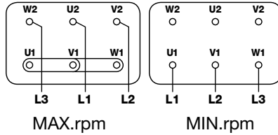
2 SPEED MOTOR (DAHLANDER WINDING)
