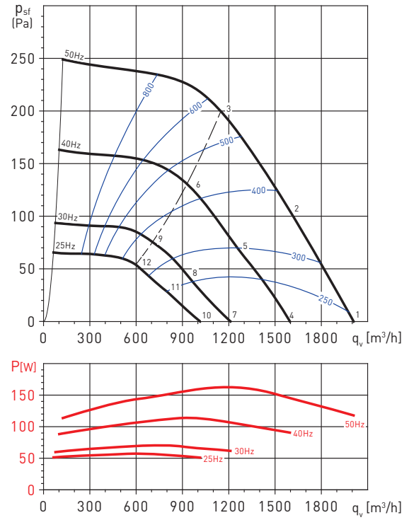
CTHT/4-225N
