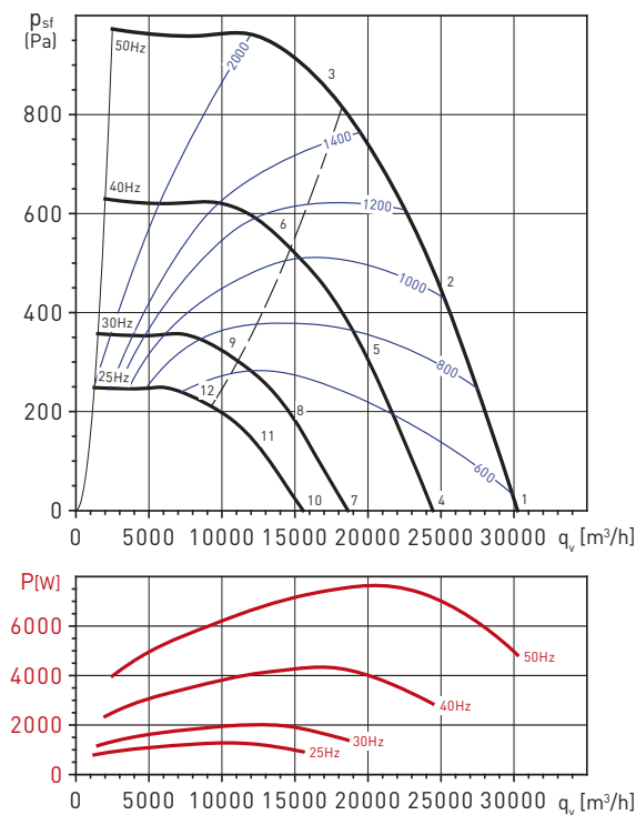
CTHT/6-710N
