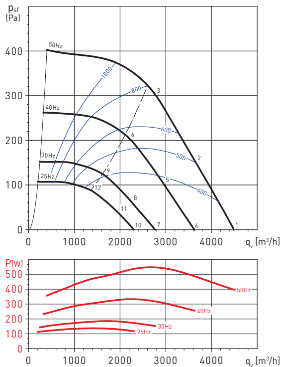
CTHT/4-315N
