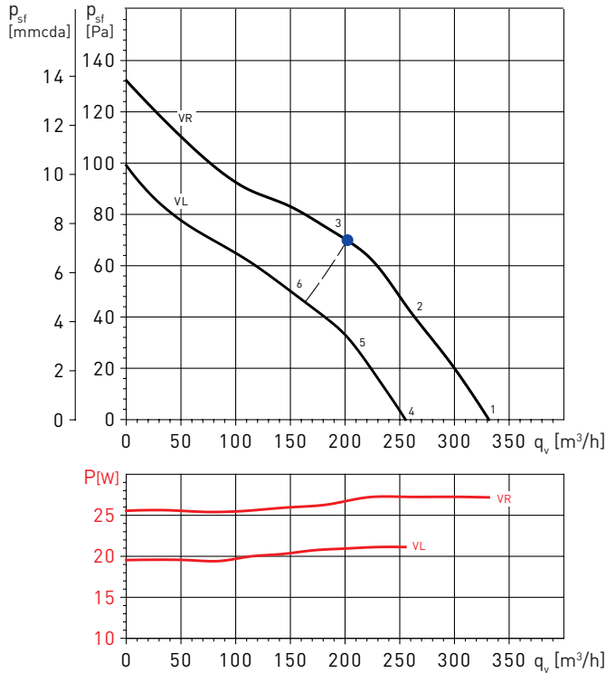
TD-350/125 SILENT
