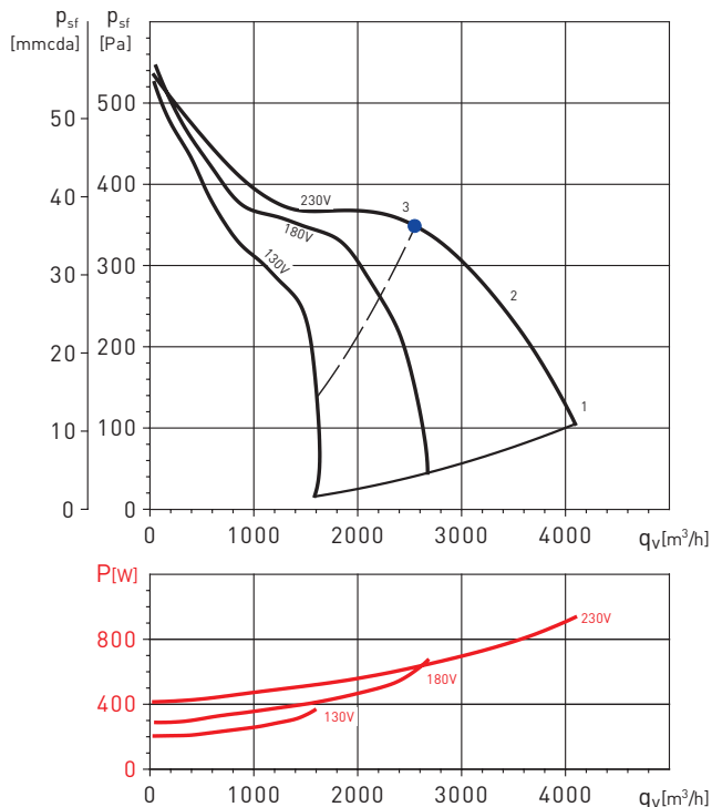
CVB/4-240/240 NT 550W
