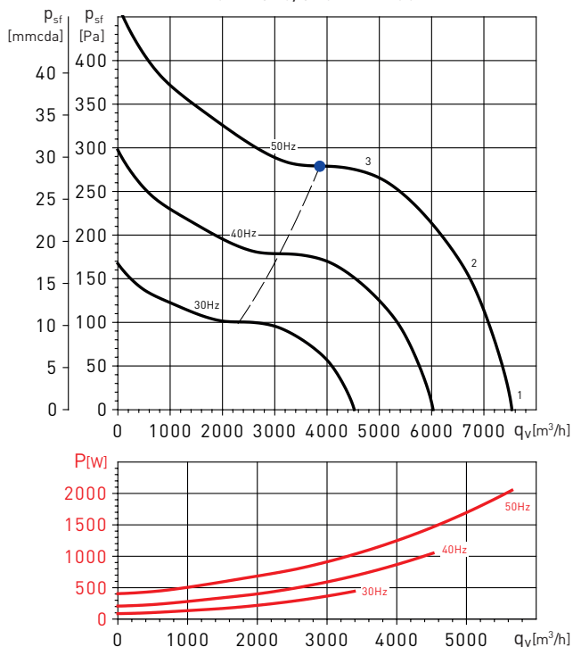
CVT-320/320 NT 1100W
