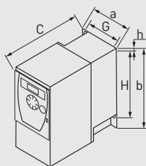
Configuration of models VFTM650 TRI 11 and 15 IP55
