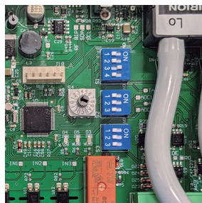
The ECOWATT PLUS ELECTRONICS allow adjusting parameters and modifying operating modes through a potentiometer and relays.
