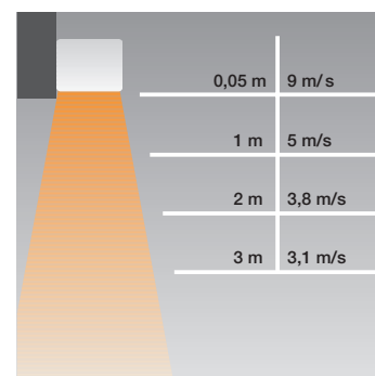
Air distance/speed
